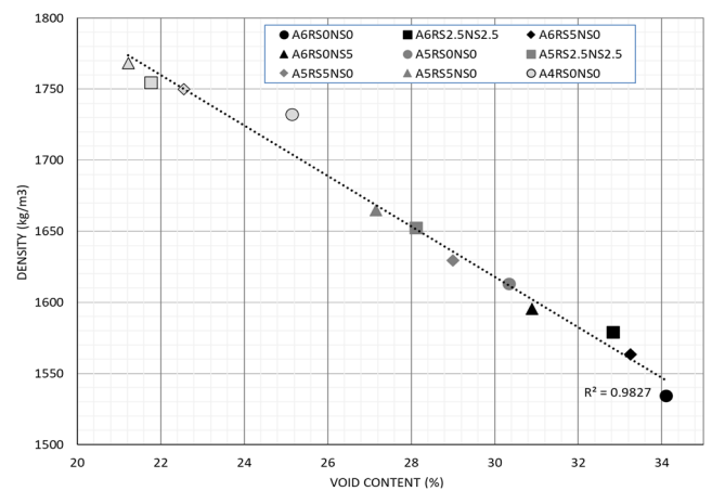
Fig. 5 Dry density vs. void content link for pervious concrete
