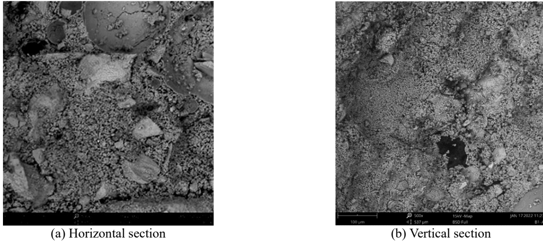
Fig. 3 Typical SEM images of the reconstituted samples
