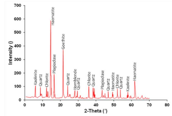
Fig. 4 XRD spectrum showing mineralogy
