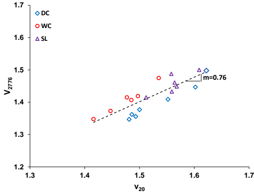
Fig. 8 Degree of convergence for samples (T-1) at 2776 kPa
