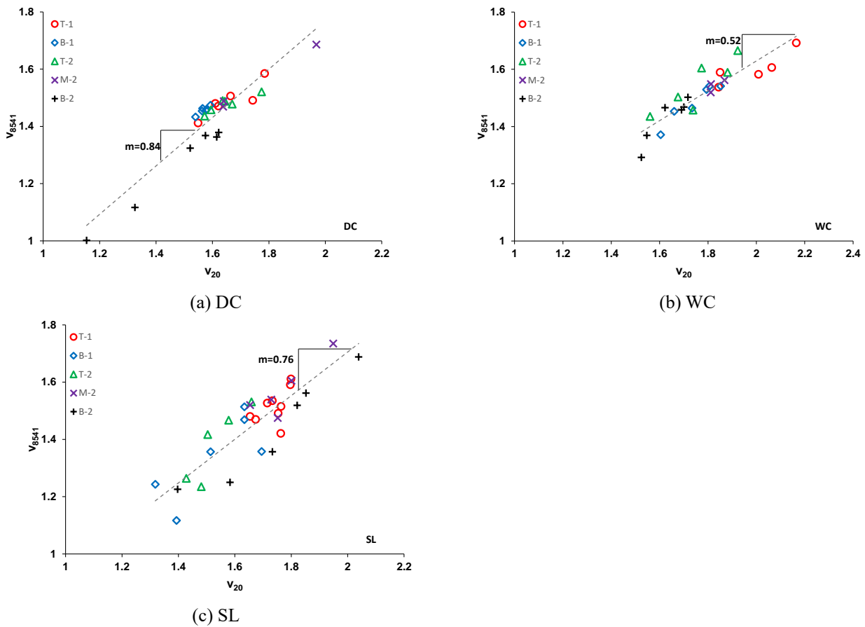
Fig. 10 Degree of convergence for different sample preparations
