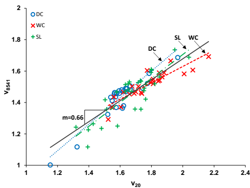
Fig. 11 Effect of sample preparations on the convergence and the overall degree of convergence for the iron tailings
