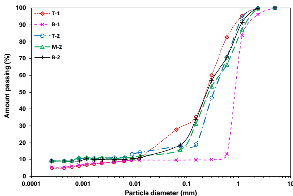
Fig. 2 Grading curves of the samples
