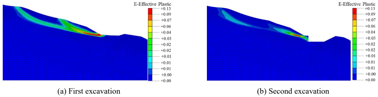
Fig. 8 Variation in the plastic zone of the slope
