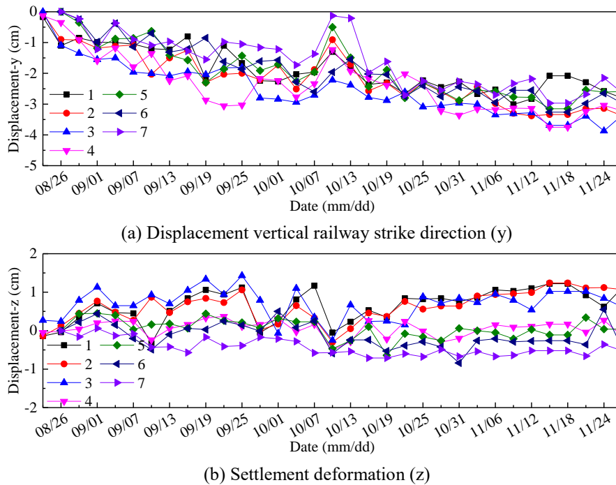
Fig. 13 Monitoring results of the displacement of the top beam
