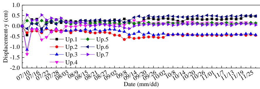
(a) Upper slope displacement vertical railway strike direction (y)
