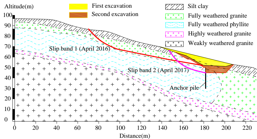
(b) Longitudinal section of the slope
