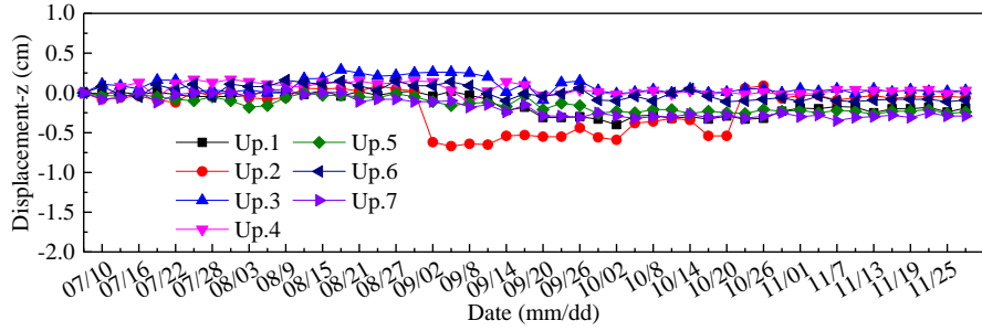
(b) upper slope settlement deformation (z)
