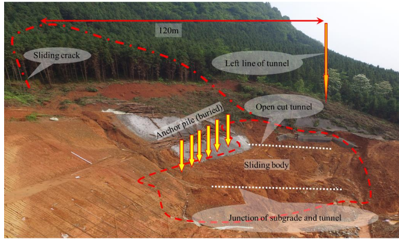
(a) Picture of the slope collapse
