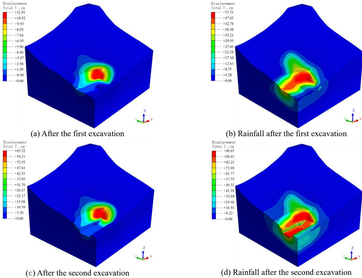
Fig. 7 Slope deformation under different working conditions
