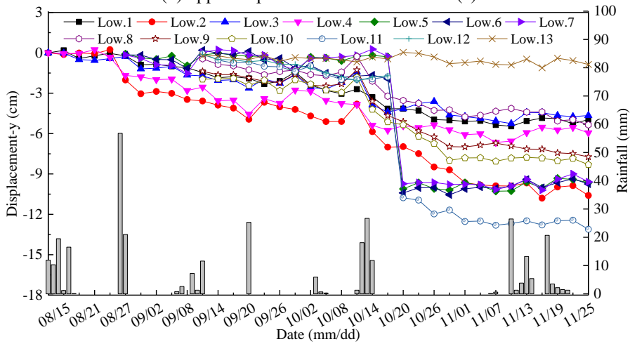
(c) Lower slope displacement vertical railway strike direction (y)
