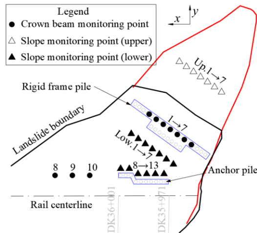
Fig. 12 Layout of displacement monitoring points on slope and anti-sliding pile
