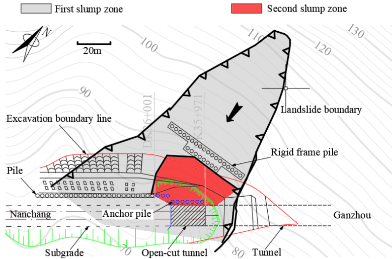
Fig. 11 Design of reinforcement measures
