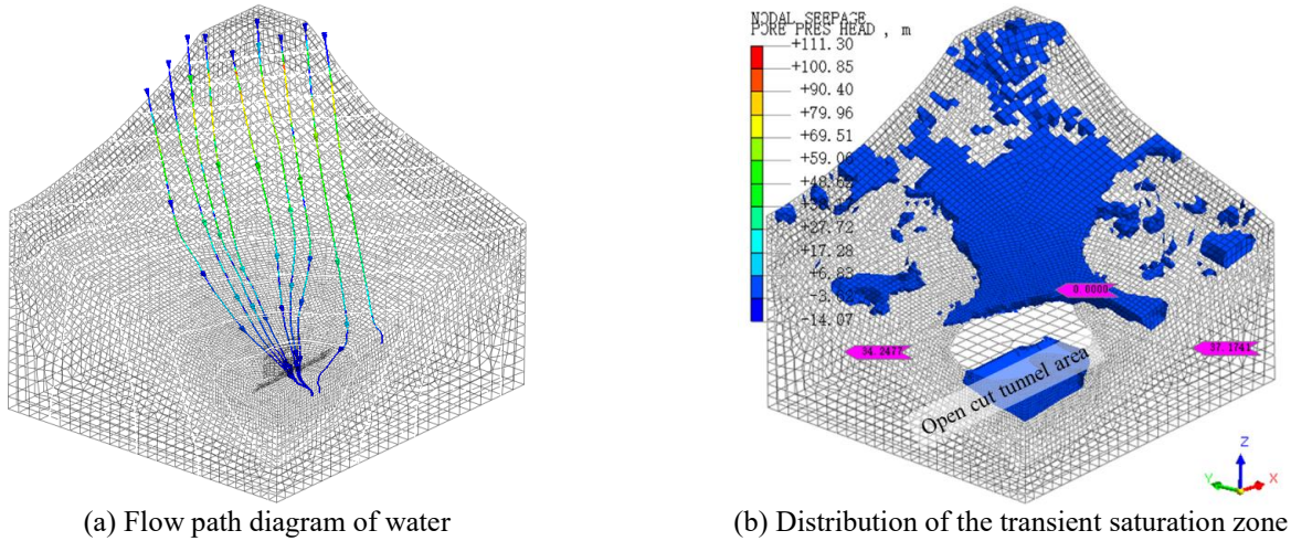
Fig. 6 Distribution of flow path and transient saturation zone
