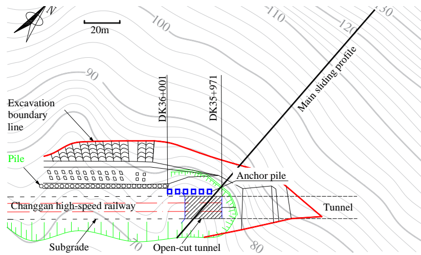
(a) Original design of the slope
