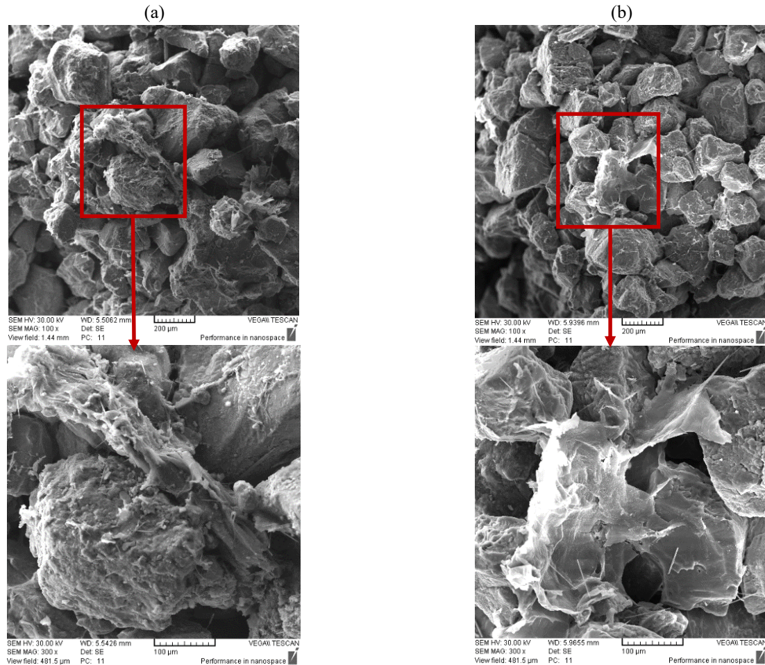
Fig. 12 SEM images of the specimens with (a) 1% and (b) 2% of serish
