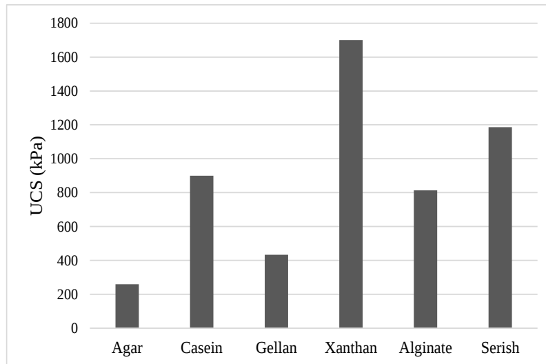
Fig. 9 Maximum UCS value of treated sand with 2% of different biopolymers (Khatami and O'Kelly 2013, Chang et al. 2015, Chang et al. 2016, Fatehi et al. 2018, Fatehi et al. 2019, Fatehi et al. 2021)
