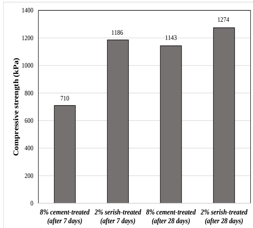
Fig. 13 Comparison of compressive strength of serish-treated sand to that of 8% cement-treated sand (after 7 and 28 days)
