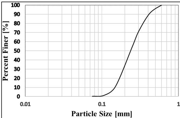
Fig. 2 Particle size distribution curve of the soil used in the study
