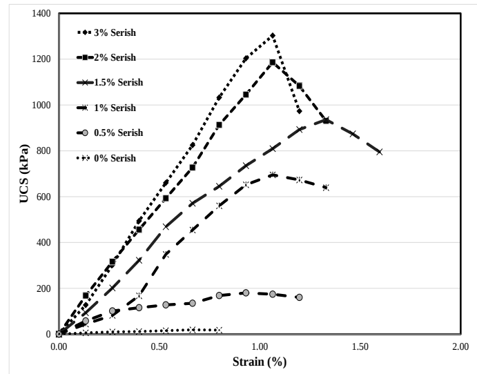
Fig. 7 Stress – axial strain curves of tested samples obtained via unconfined compression test
