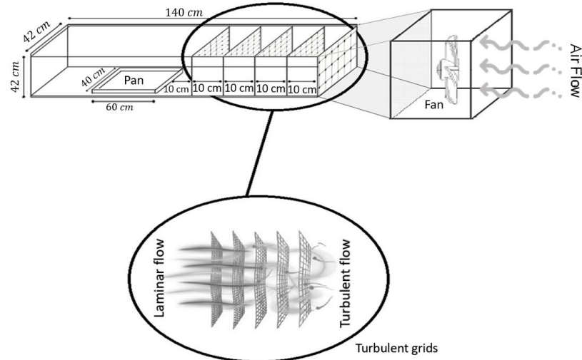
(b) Schematic view for the detail configuration
