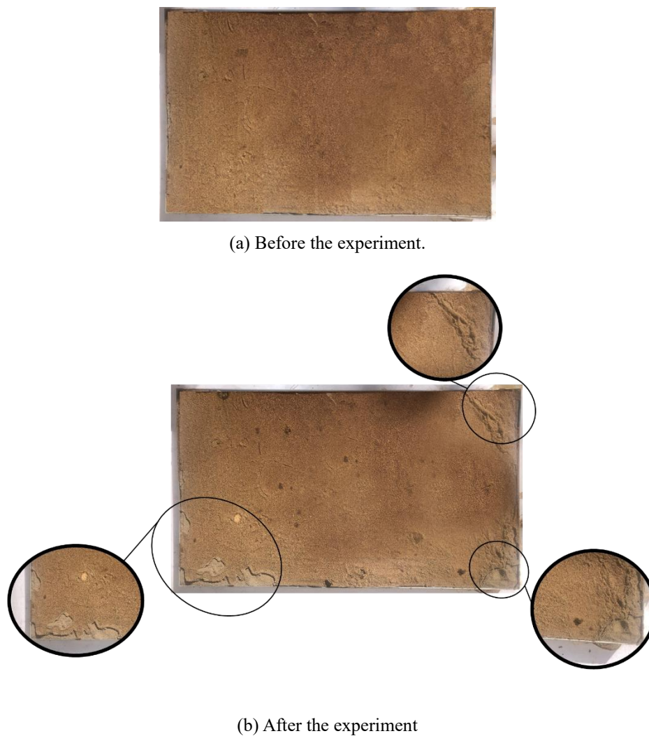
Fig. 11 Serish-treated sand sample for the wind erosion test
