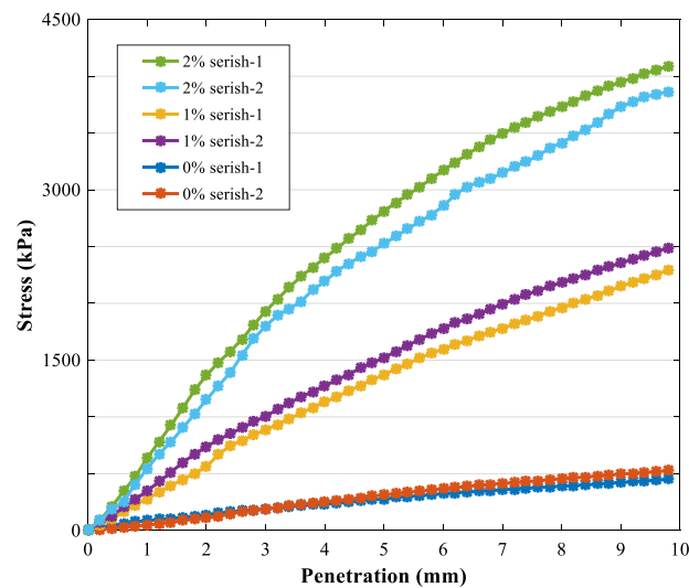
(a) Stress-penetration curves
