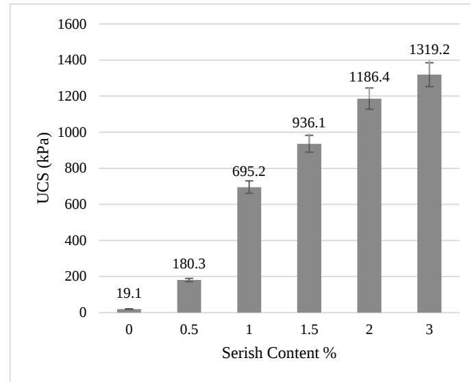
Fig. 8 The unconfined compressive strength variation with serish contents
