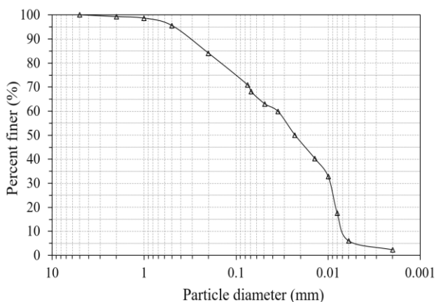
Fig. 1 Particle size distribution of soil sample (Chen et al. 2020)
