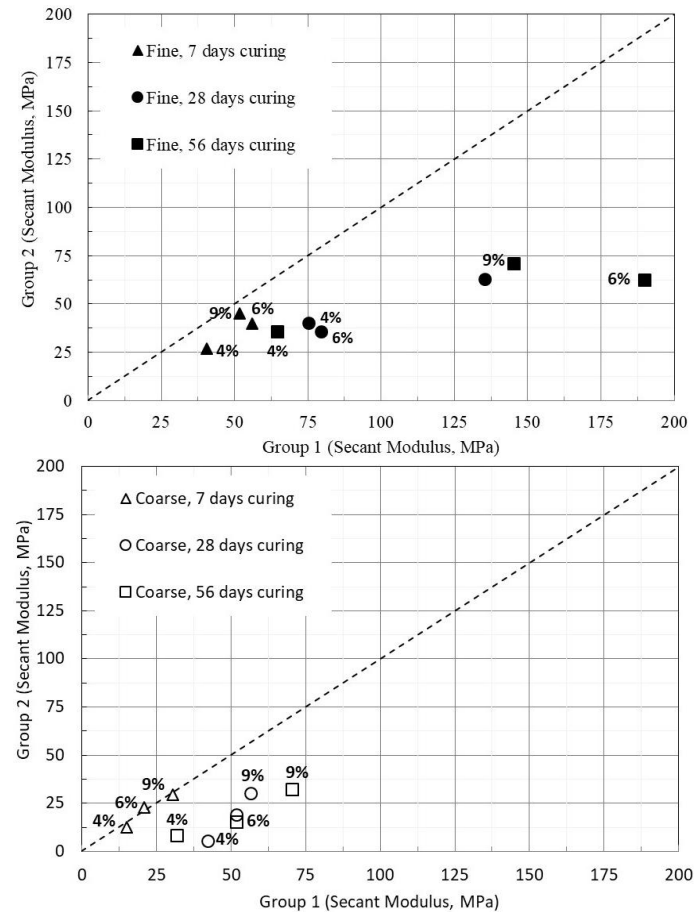
Fig. 11 Comparison of Group 1 and Group 2 samples in terms of Secant Modulus at failure values (for fine and coarse soil pulverization)
