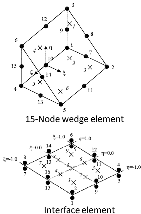
Fig. 13 The adopted 3D element in the numerical modelling
