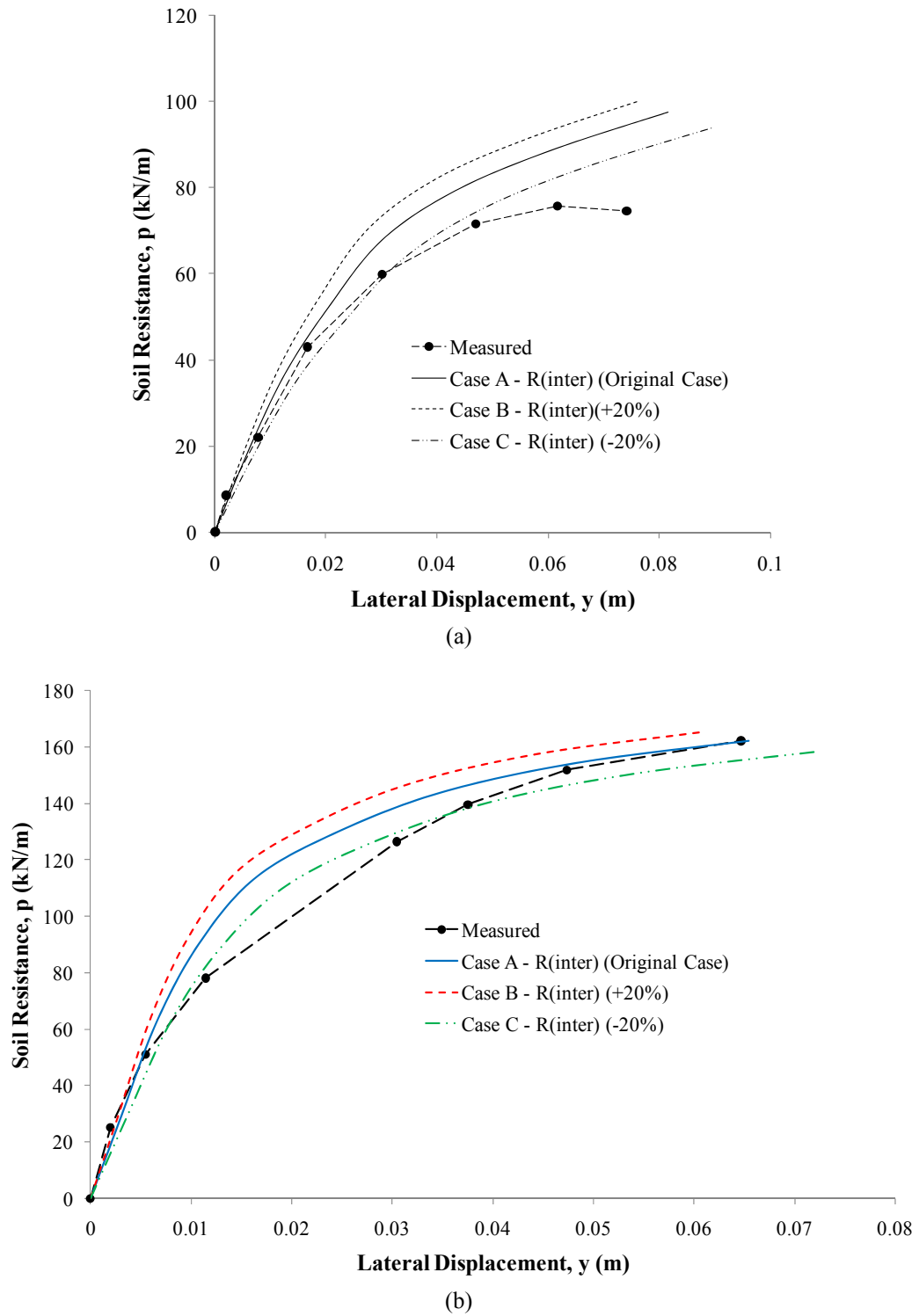
Fig. 22 Variation of p - y curves with R_{inter} at: (a) 2D depth; and (b) 4D depth ( D = pile diameter)
