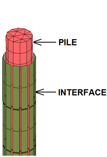
Fig. 11 Interface arrangement around the pile in the finite element model
