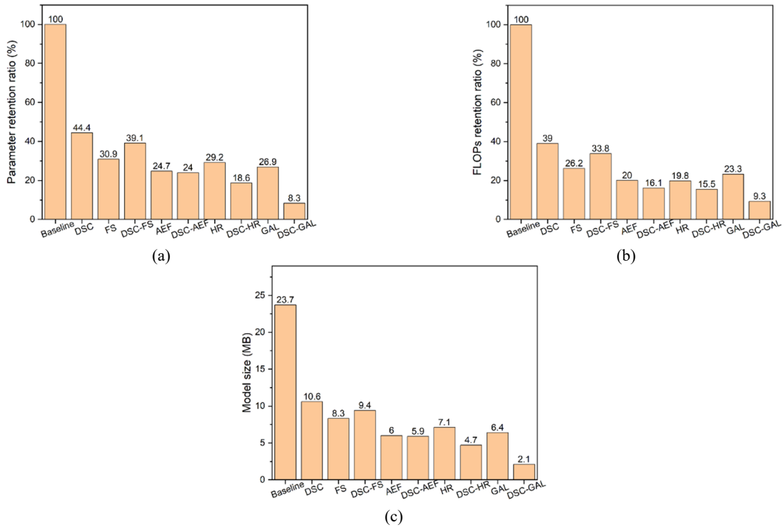
Fig. 10 (a) Parameter retention ratio; (b) FLOP retention ratio; and (c) model size for different hybrid compression strategies.
