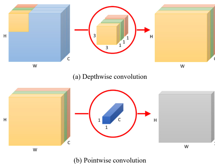
Fig. 1 Depthwise separable convolution
