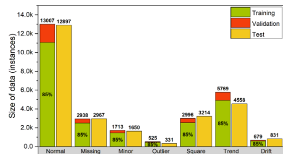
Fig. 6 Size of data for different types of data anomalies
