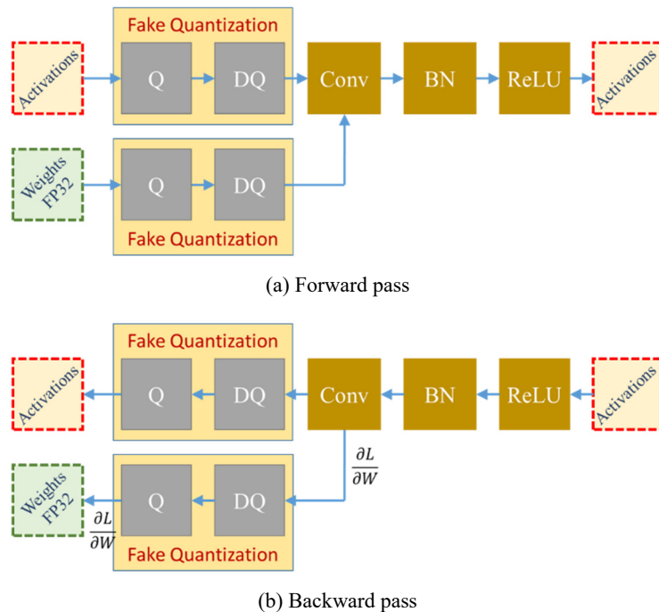
Fig. 2 Fake quantization in forward and backward passes; Q: Quantization; DQ: De-quantization; Conv: Convolution; BN: Batch Normalization; ReLU: Rectified Linear Unit; L: Loss; W: Weights
