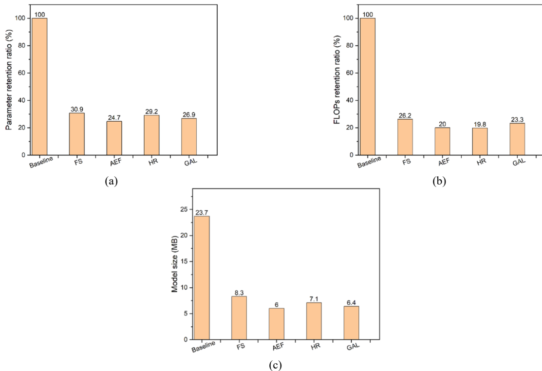
Fig. 9 (a) Parameter retention ratio; (b) FLOP retention ratio; and (c) model size for different pruning techniques
