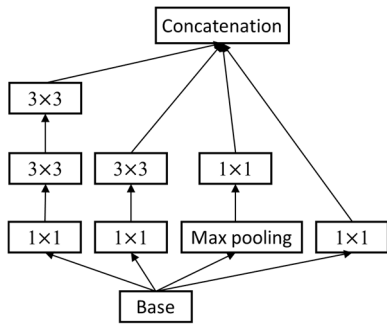
Fig. 7 Inception module used in GoogLeNet
