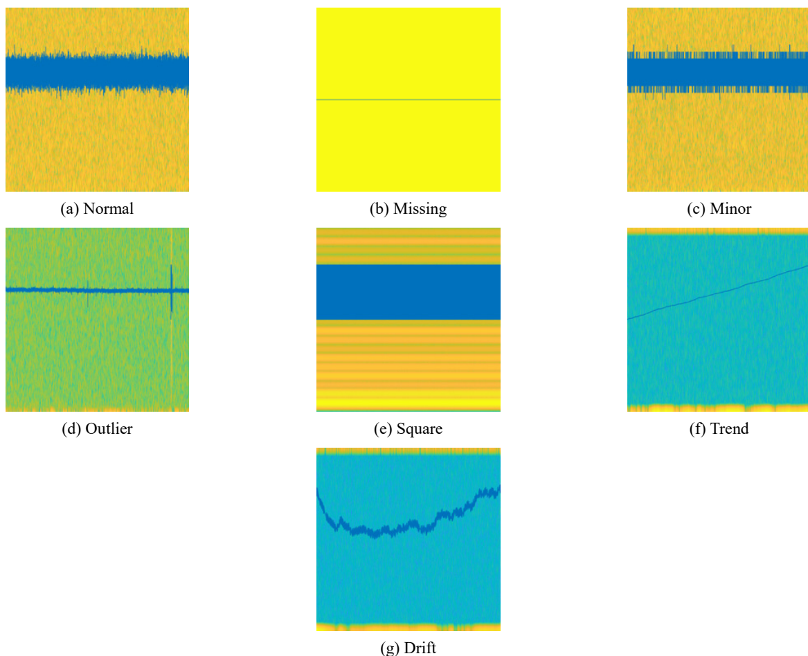
Fig. 8 Time-frequency representation of different types of data anomalies
