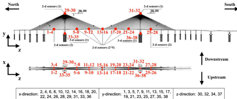
Fig. 4 Depiction of sensor locations used for data acquisition (Bao et al. 2021)
