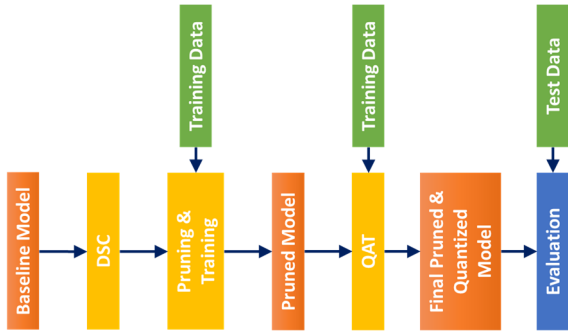
Fig. 3 An overview of the proposed three-pronged network compression approach; DSC: depthwise separable convolution; QAT: quantization-aware training
