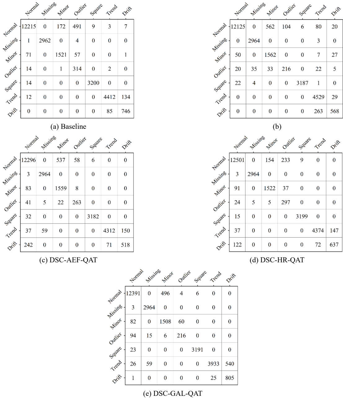
Fig. 11 Confusion matrices corresponding to the baseline and compressed models
