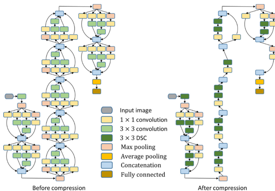
Fig. 13 A depiction of the GoogLeNet architecture before and after the application of the hybrid compression technique
