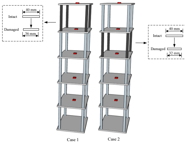
Fig. 14 Two damage cases of steel frame model
