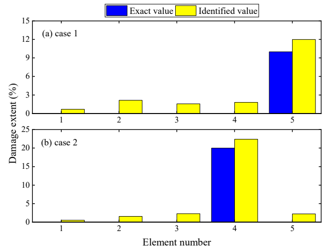
Fig. 15 Identified damage extent with output-only responses: (a) case 1; (b) case 2
