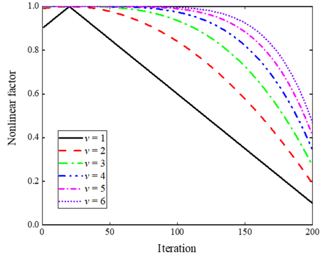
Fig. 2 The variation curves of nonlinear factor for different power exponents
