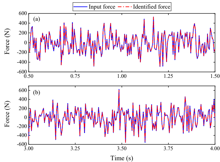
Fig. 8 The identified force time histories of truss structure for noise free case: (a) 0.5-1.5 s; (b) 3.0-4.0 s
