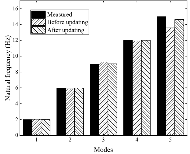
Fig. 13 The measured and updated natural frequencies of five-floor frame model
