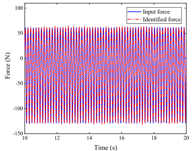
Fig. 16 Comparison of measured and identified input excitation from 10 to 20 s in damage case 2
