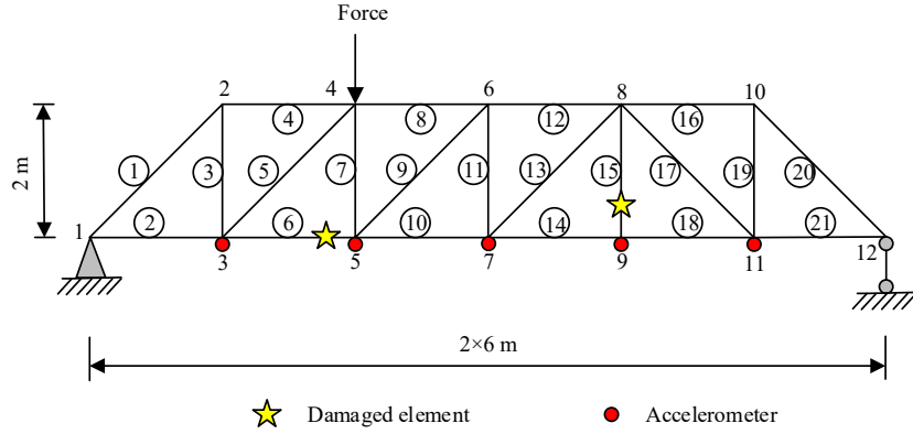
Fig. 5 The numerical model of a plane truss structure
