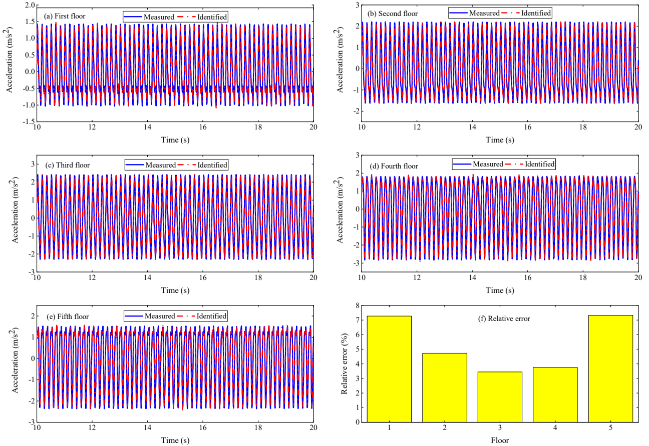
Fig. 17 The measured and predicted acceleration time histories of frame model in case 2: (a) first floor; (b) second floor; (c) third floor; (d) fourth floor; (e) fifth floor; (f) relative error
