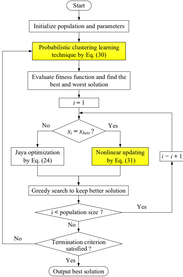
Fig. 3 The flowchart of proposed M-Jaya algorithm
