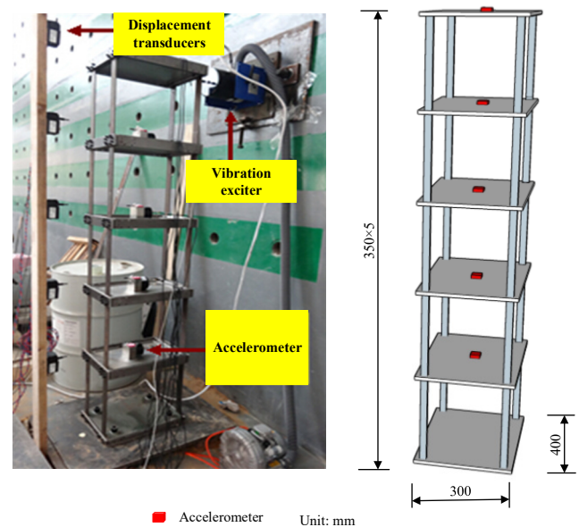
Fig. 11 Experimental tests on a five-story steel frame model
