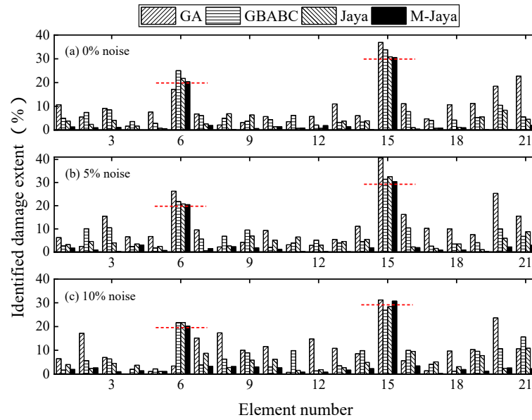
Fig. 7 Identified results of simply supported truss with four heuristic algorithms: (a) 0% noise; (b) 5% noise; (c) 10% noise
