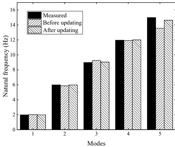
Fig. 13 The measured and updated natural frequencies of five-floor frame model
