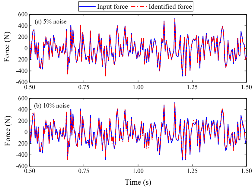
Fig. 9 The comparison between the identified and true force: (a) 5% noise; (b) 10% noise
