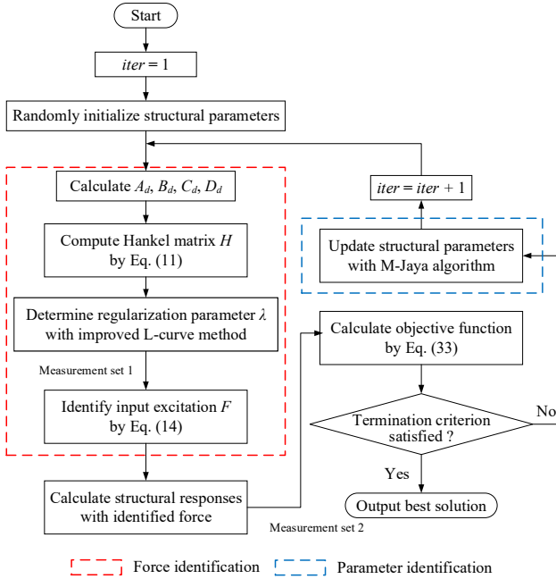
Fig. 4 The identification flowchart of structure parameters and input excitation
