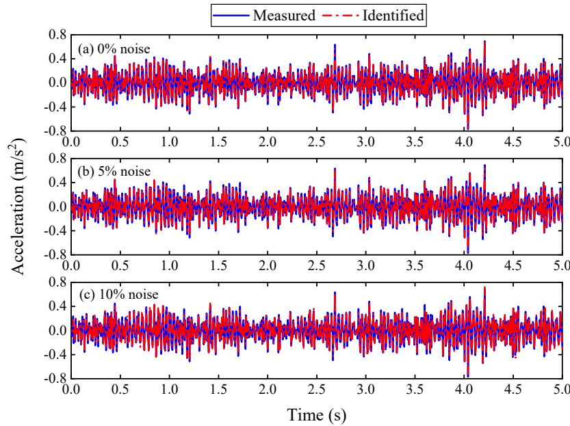
Fig. 10 The measured and predicted acceleration at node 7 under noise level: (a) 0%; (b) 5%; (c) 10%
