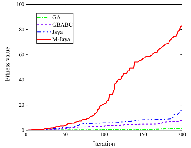
Fig. 6 Comparison of convergence for four different algorithms
