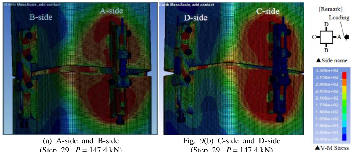
Fig. 9 von Mises stress contour plots (Step 29, P = 147.4 kN) at 90^\circ
