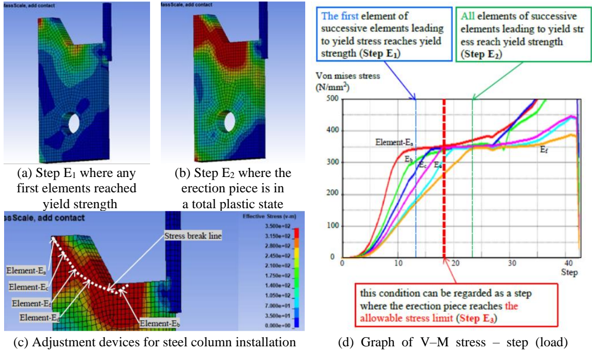
Fig. 12 Method for determining the allowable loading step at the yielding of an erection piece
