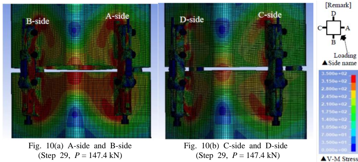
Fig. 10 von Mises stress contour plots (Step 29, P = 147.4 kN) at 45^\circ
