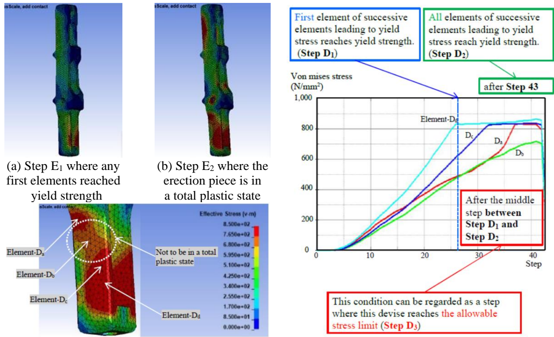
Fig. 13 Method for determining the allowable loading step at the yielding of a device for erection alignment
